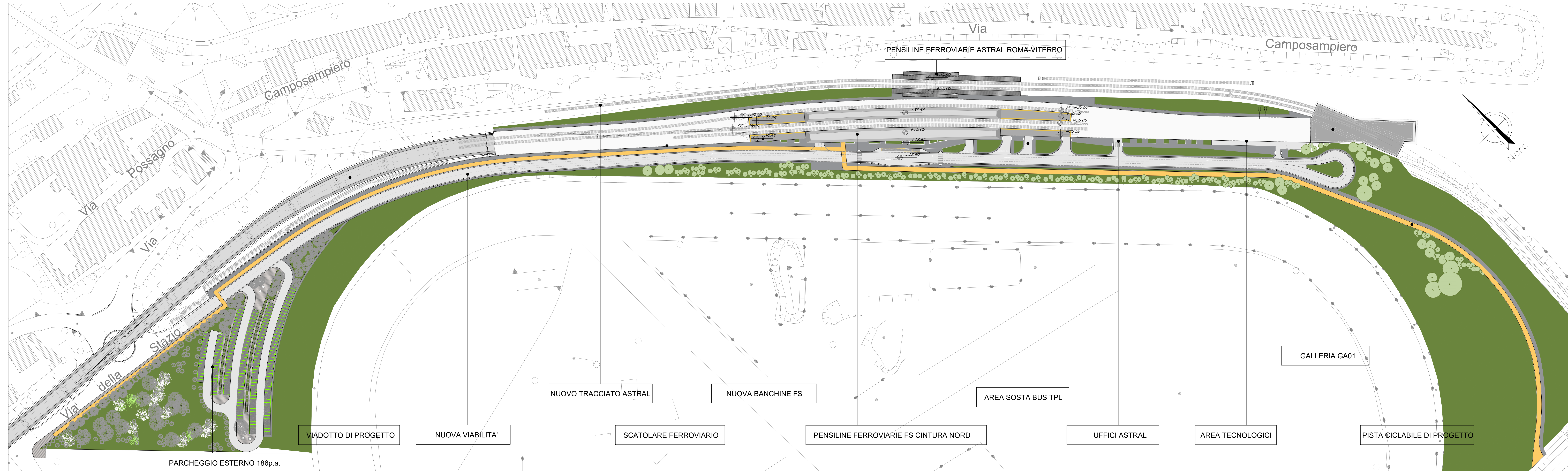
PLANIMETRIA POST OPERA scala 1:1000
