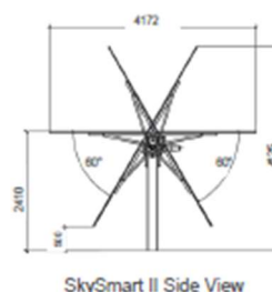
Fig. 8 – Datasheet tracker SkySmart II (ARCTECH)
