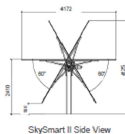
Fig. 2 – Datasheet tracker SkySmart II (ARCTECH)
