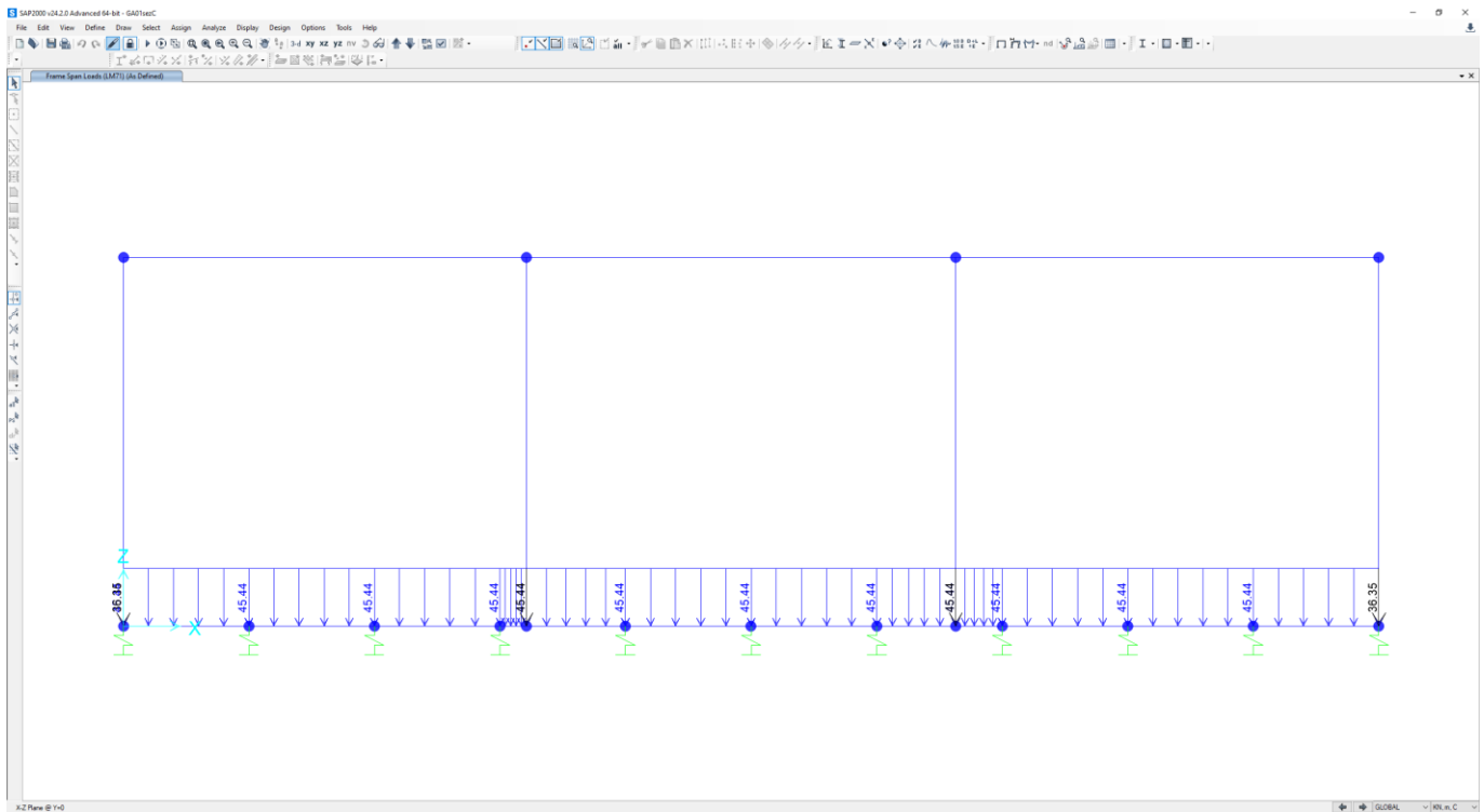
Figura 9-5: carico LM71
