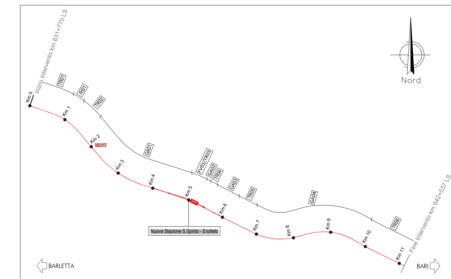
KEYPLAN
