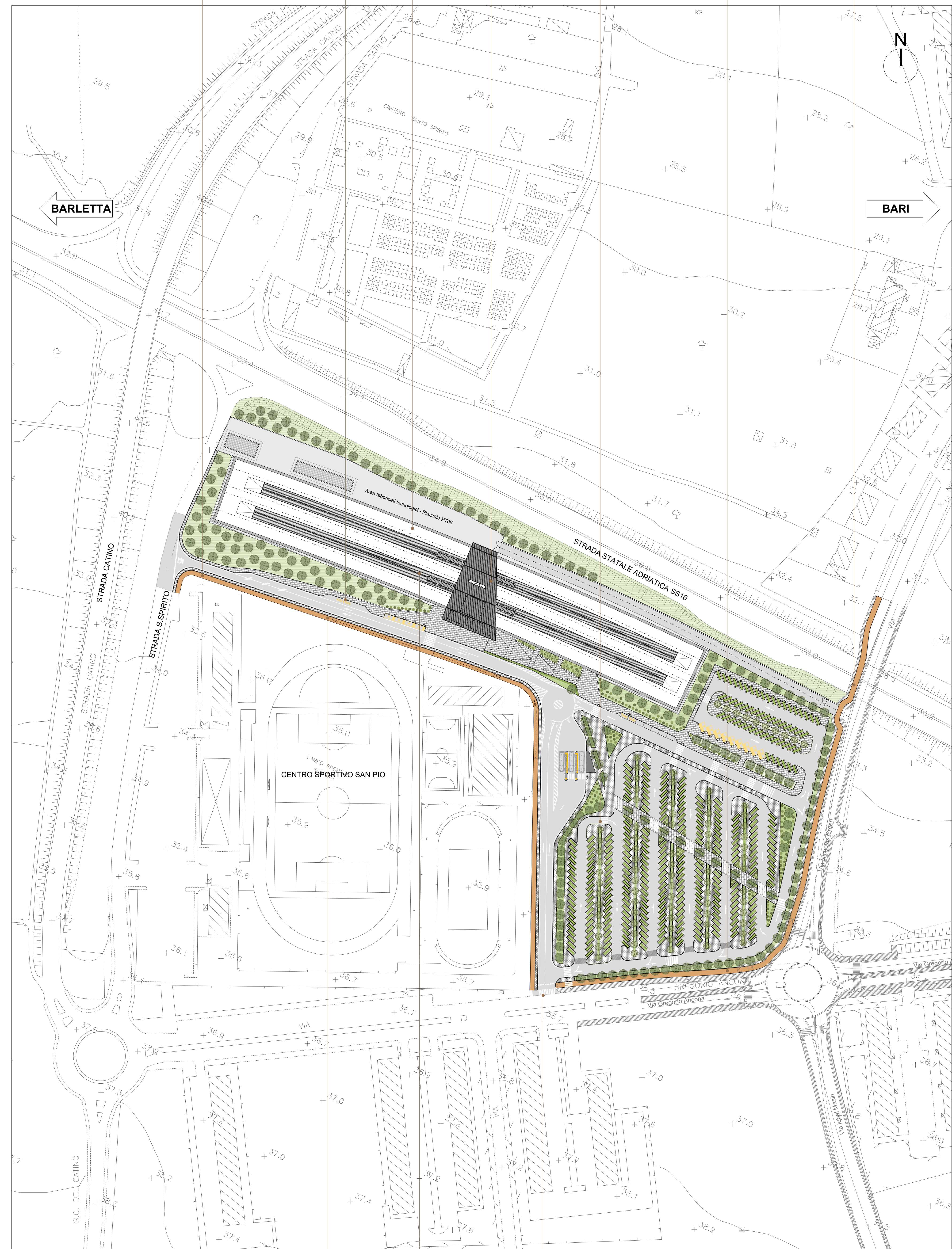
Planimetria Post Operam Scala 1:1000
