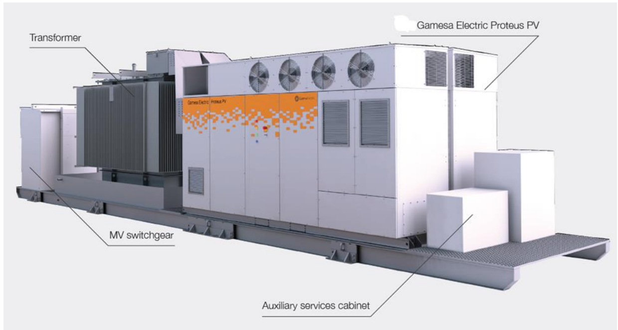
Figura 4.1 – Vista Power station
