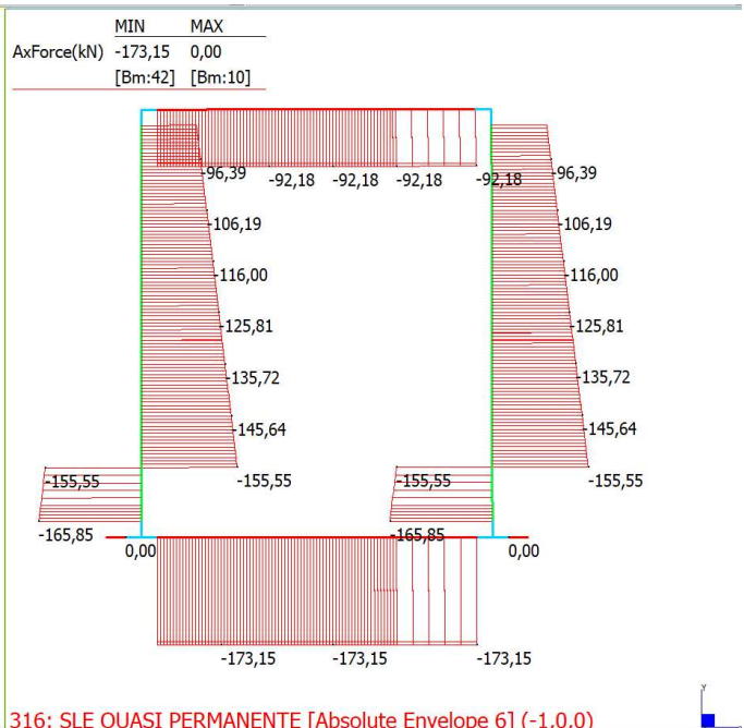
316: SLE QUASI PERMANENTE [Absolute Envelope 6] (-1.0,0)
