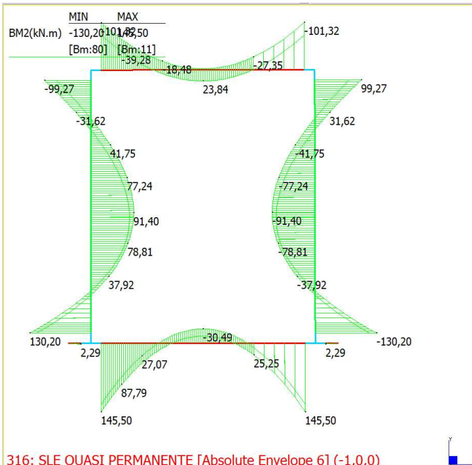
316: SLE QUASI PERMANENTE [Absolute Envelope 6] (-1.0,0)
