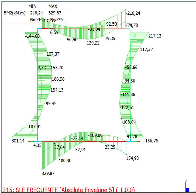
315: SLE FREQUENTE [Absolute Envelope 5] (-1.0,0)
