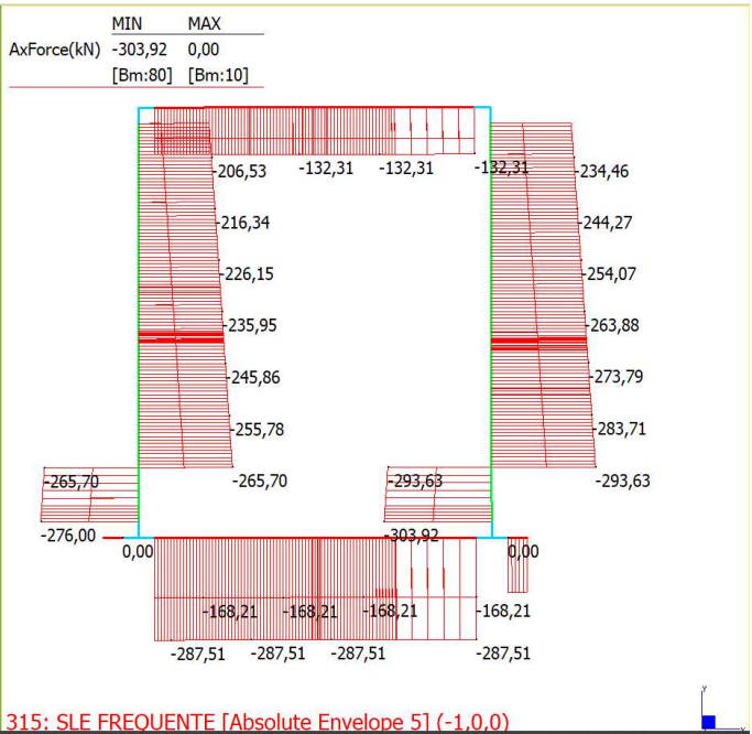
315: SLE FREQUENTE [Absolute Envelope 5] (-1.0,0)
