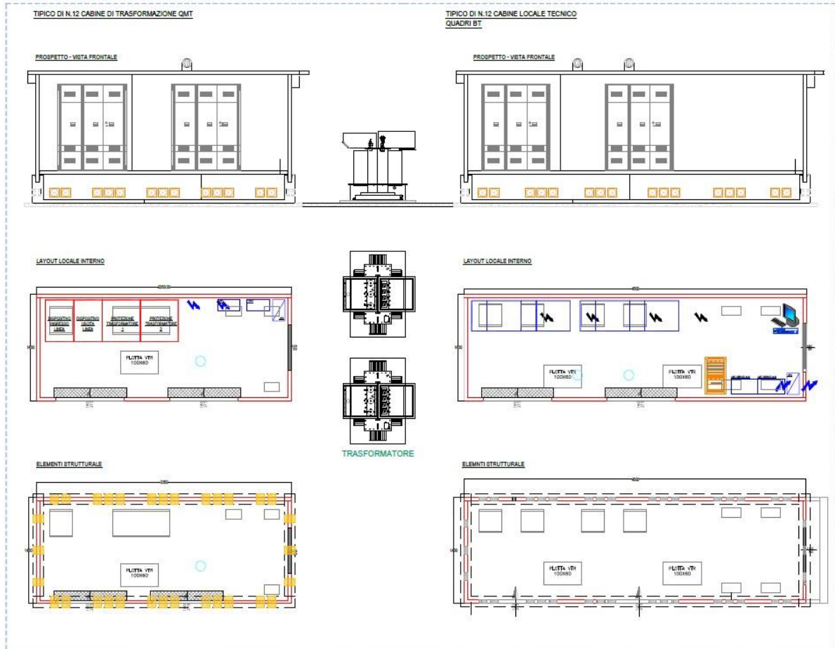
Figura 2.1: Power Station
