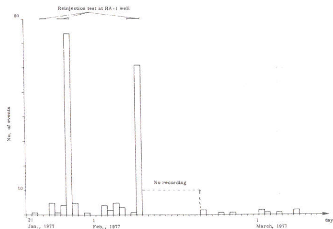
Fig. 4. Torre Alfina area - histogram of seismic events recorded by provisional network during some reinjection tests at RA-1 well.
