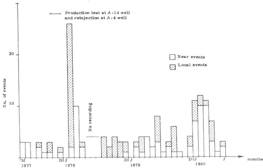
Fig. 2. Torre Alfina area - histogram of seismic events recorded by permanent network.
