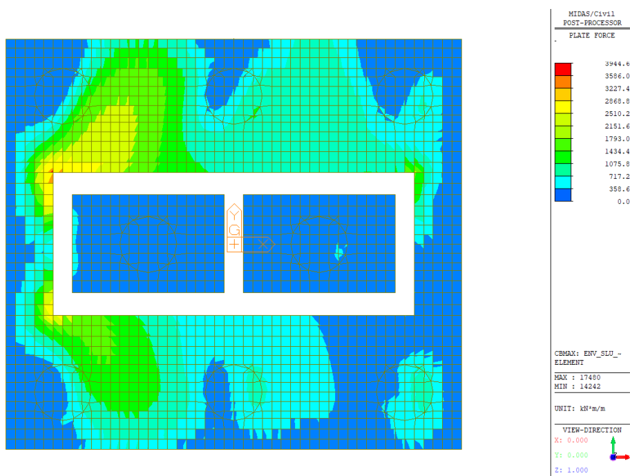
Figura 35 – Wood Armer Moment – Direction1 – Bottom (Inviluppo SLU/SLV)
