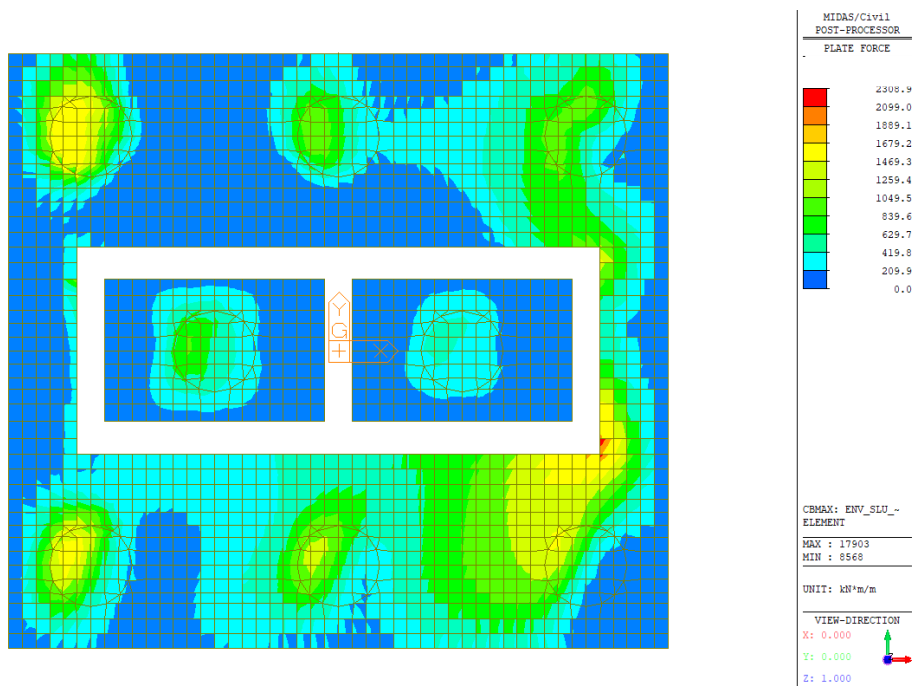
Figura 34 – Wood Armer Moment – Direction1 – Top (Inviluppo SLU/SLV)
