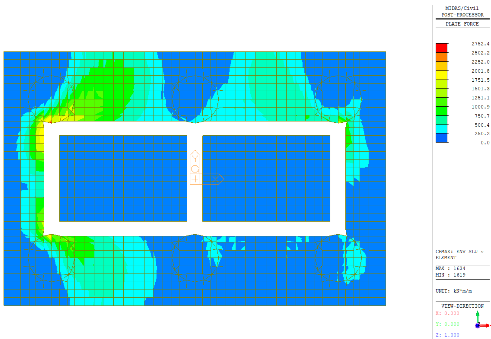
Figura 33 – Wood Armer Moment – Direction1 – Bottom (Inviluppo SLU/SLV)
