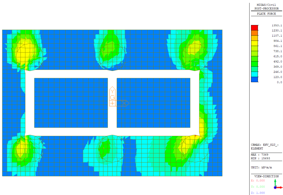
Figura 32 – Wood Armer Moment – Direction1 – Top (Inviluppo SLU/SLV)
