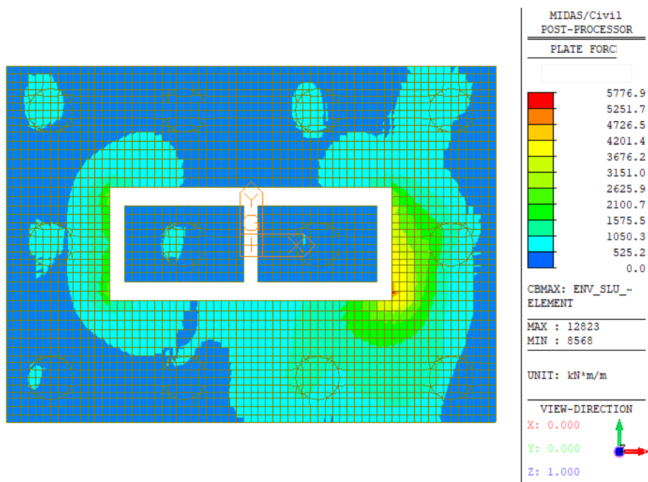
Figura 32 – Wood Armer Moment – Direction1 – Top (Involuppo SLU/SLV)
