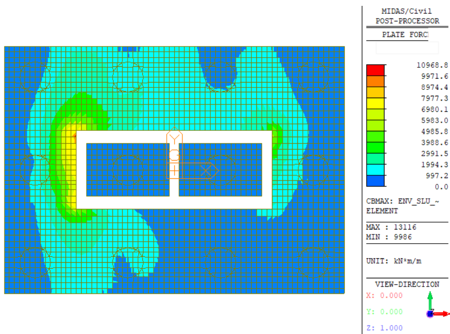
Figura 33 – Wood Armer Moment – Direction1 – Bottom (Involuppo SLU/SLV)
