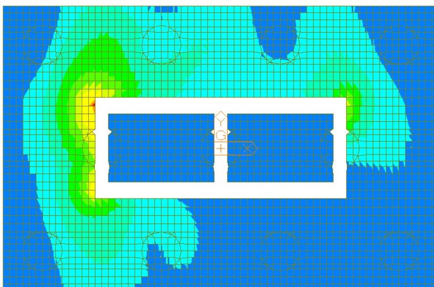
Figura 33 – Wood Armer Moment – Direction1 – Bottom (Involuppo SLU/SLV)
