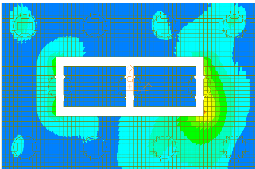
Figura 32 – Wood Armer Moment – Direction1 – Top (Involuppo SLU/SLV)
