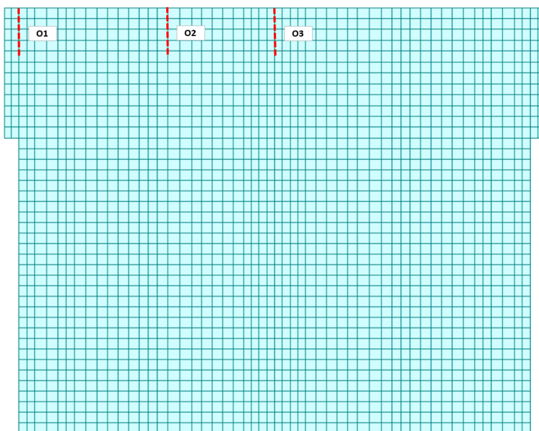
Figura 66 – Section-cut verticali trave paraghiaia
