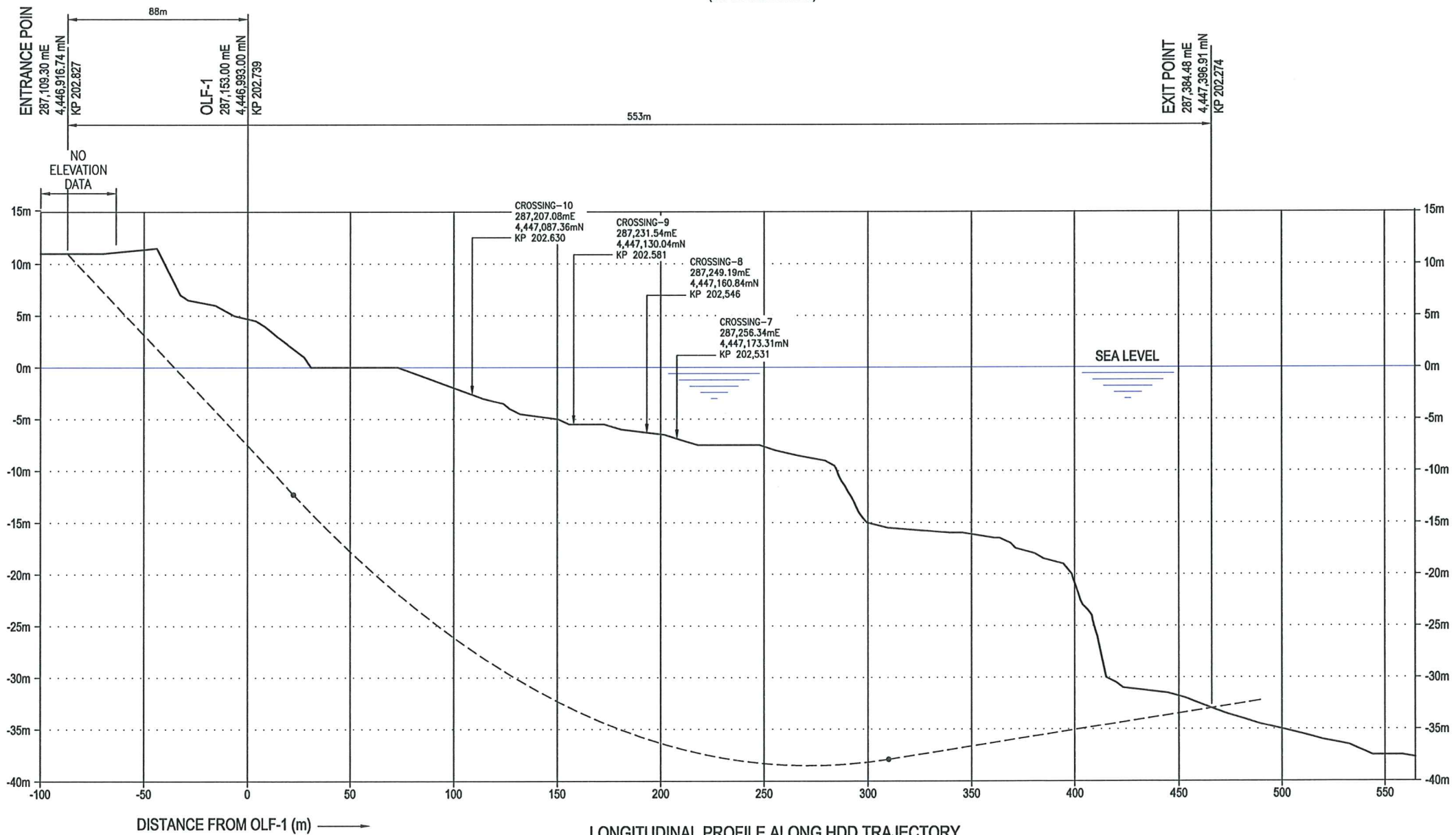
LONGITUDINAL PROFILE ALONG HDD TRAJECTORY (VERTICAL EXAGGERATION = 5x)
