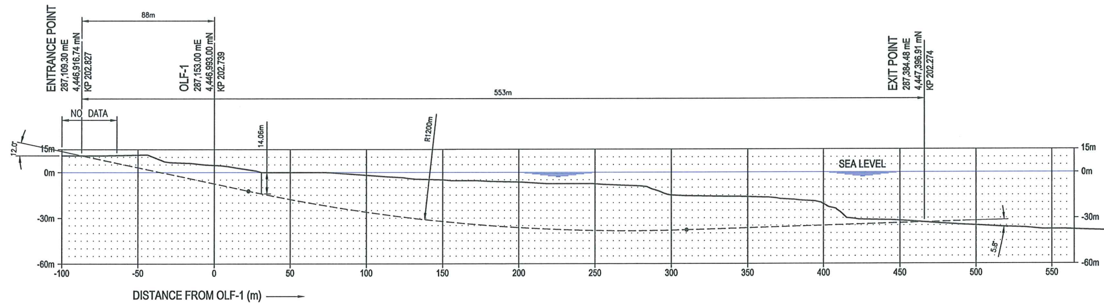
LONGITUDINAL PROFILE ALONG HDD TRAJECTORY (NO EXAGGERATION)
