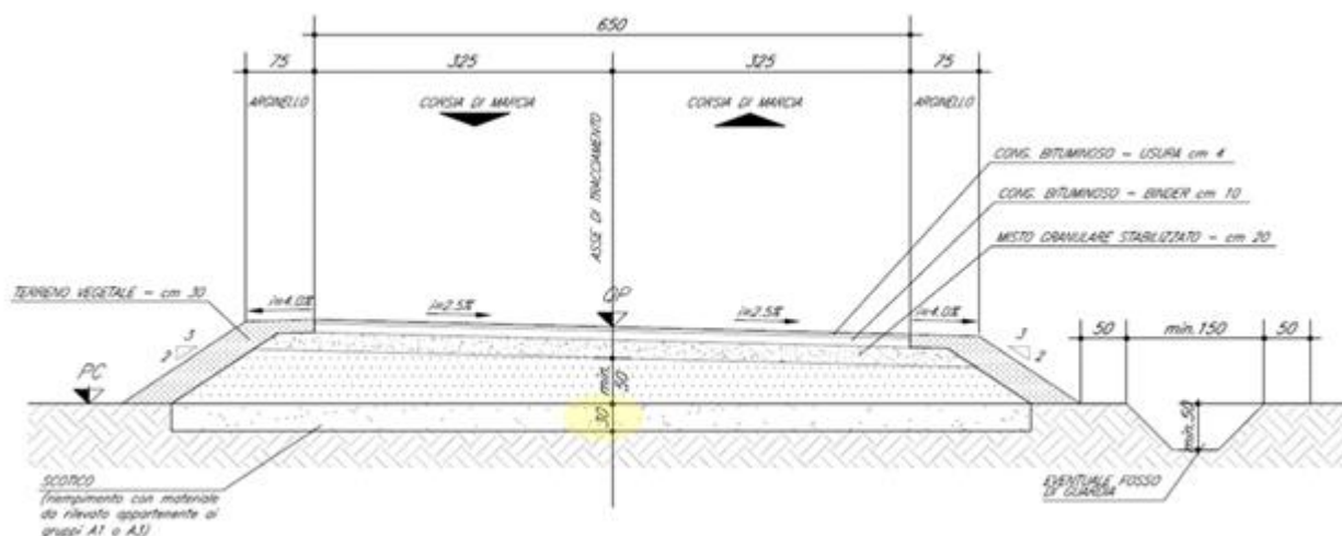
Estratto planimetria INOR11EE2PZGA1707001A
