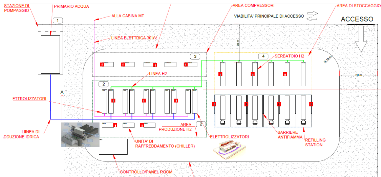
Fig. 3.23 – Layout dell’impianto Power to Gas
