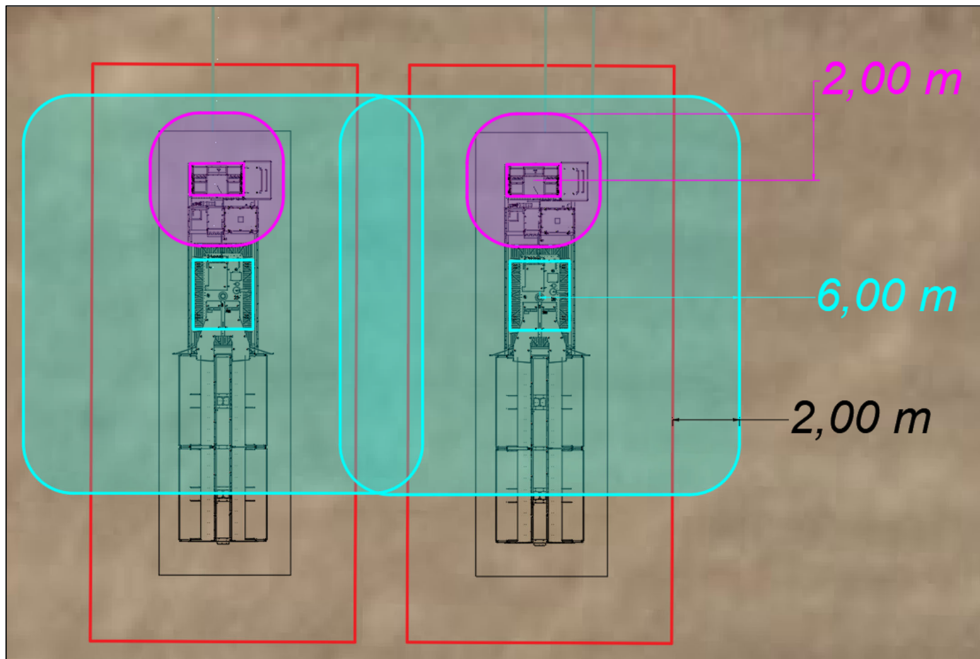
Figura 8 DRS POWER STATION (PS9)
