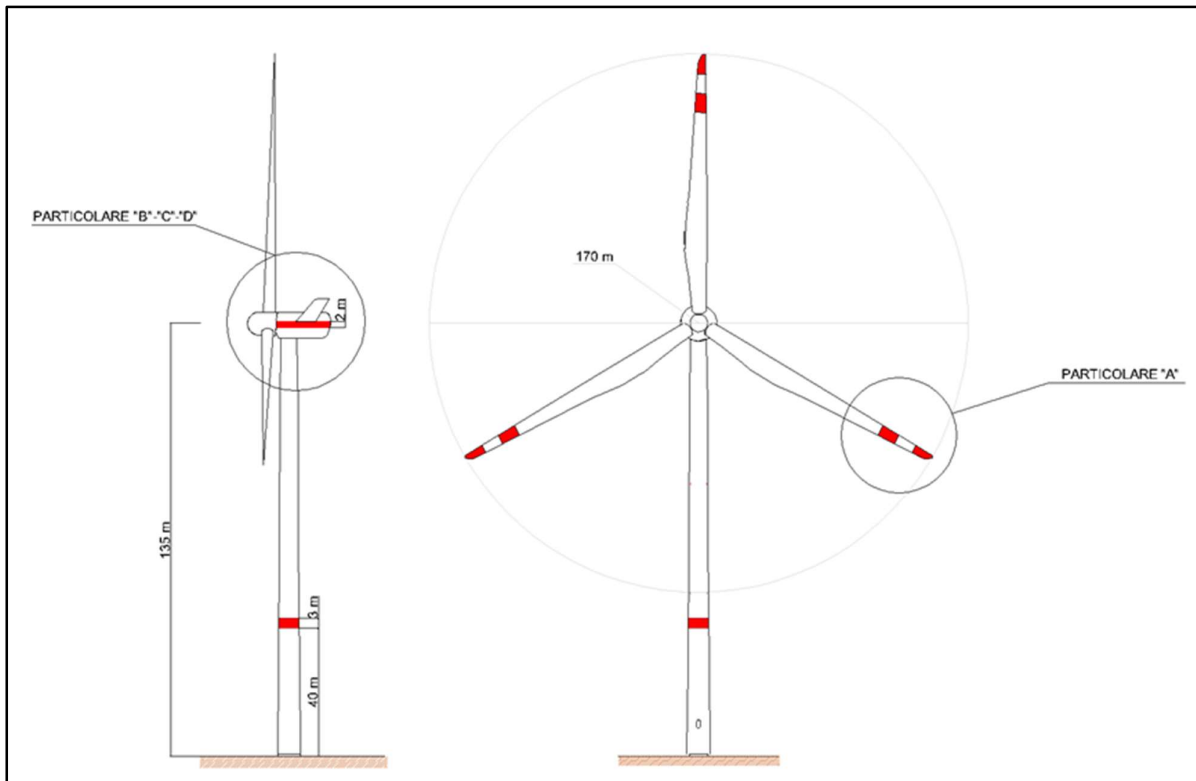
Figura 6.1.1: Profilo aerogeneratore SG170 – 6,0 MW – HH = 135 m – D = 170 m
