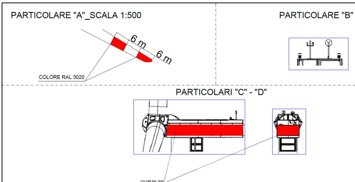
Figura 6.1.2: Particolari aerogeneratore SG170 – 6,0 MW – HH = 135 m – D = 170 m
