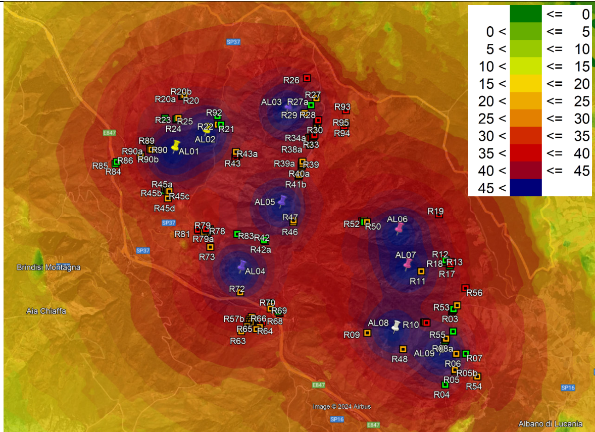
Siemens Gamesa SG 6.0 - D170 - H135: Sound Power Levels [106,0 dBA]- MAPPA VELOCITA' 12ms
