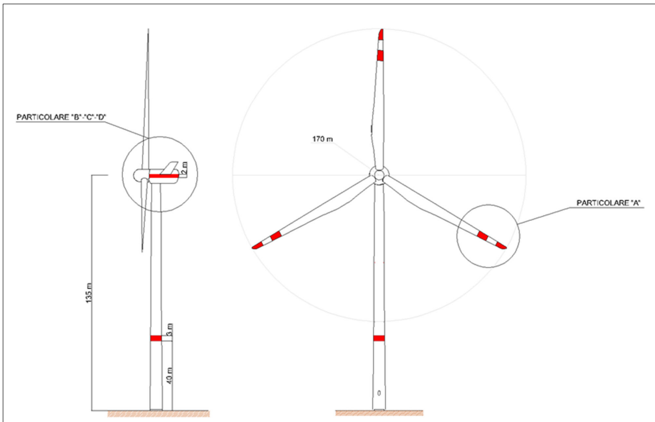
Figura 2.1: Profilo aerogeneratore SG170 – 6,0 MW – HH = 135 m – D = 170 m
