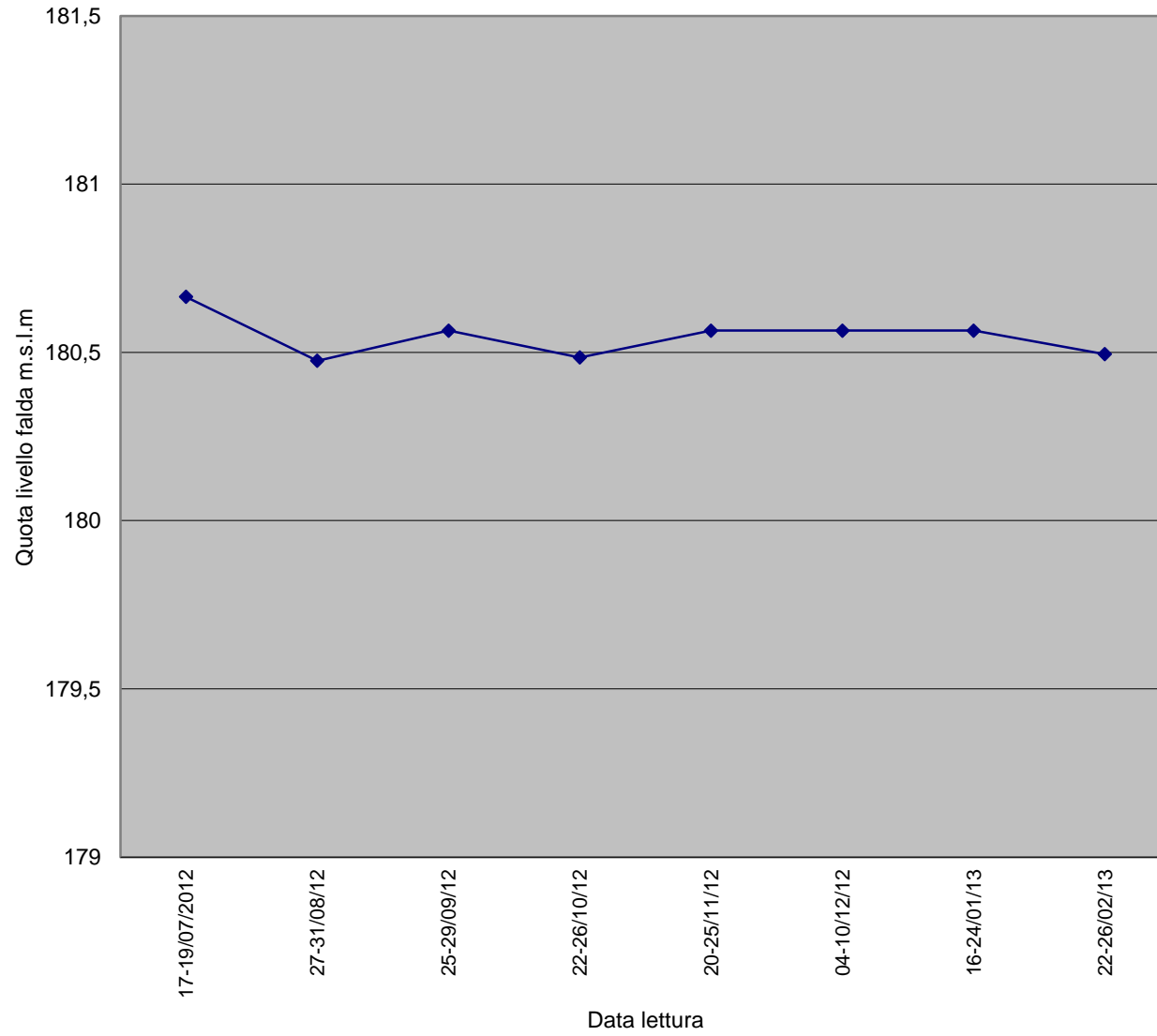
IOV-RO-010 (q.p.c 184,605)
