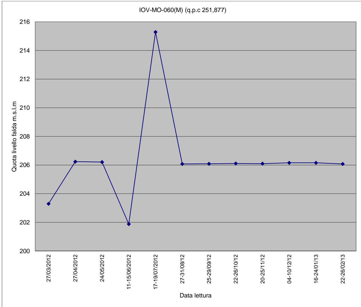
Piezometro IOV-MO-060(M)
