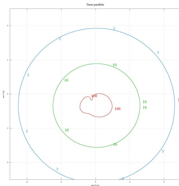
Isolinee - 4 linee MT in trincea a 25cm
