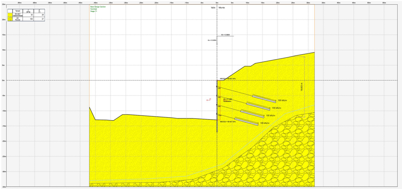
Figura 8.8 Stage 11
