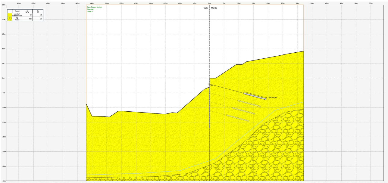
Figura 8.4 Stage 3
