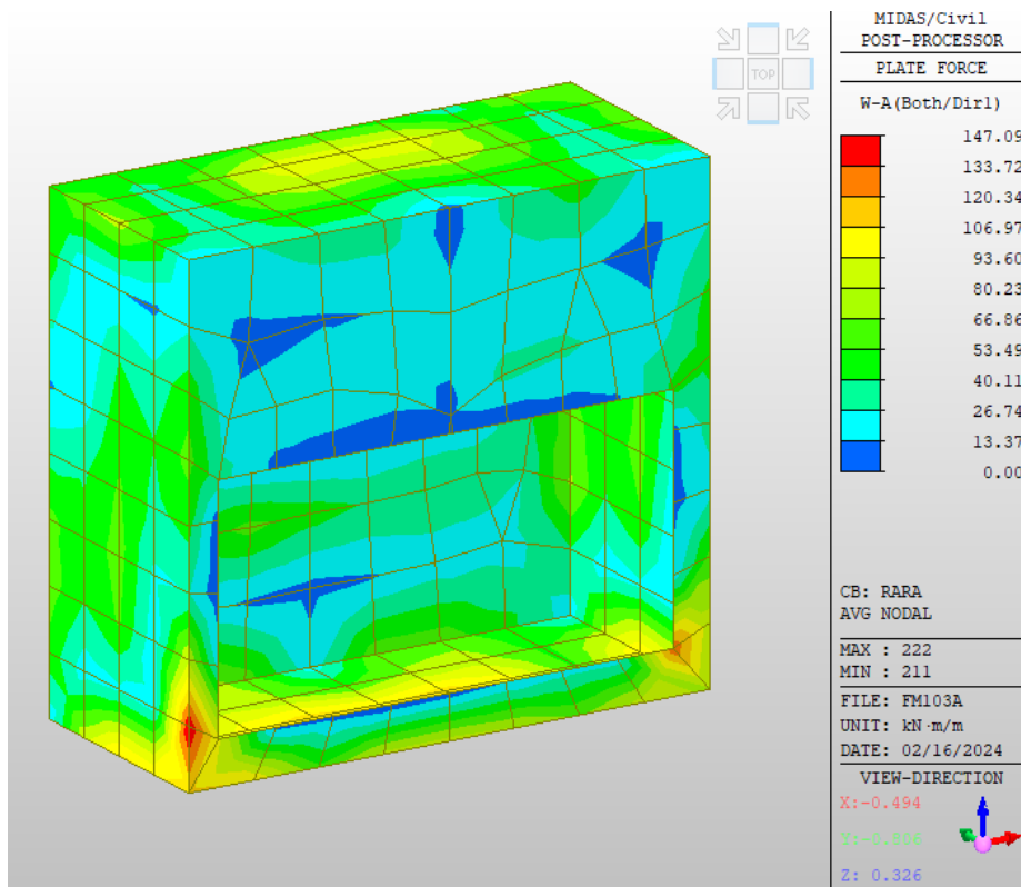
Figura 15 Wood e Armer dir 1 SLE
