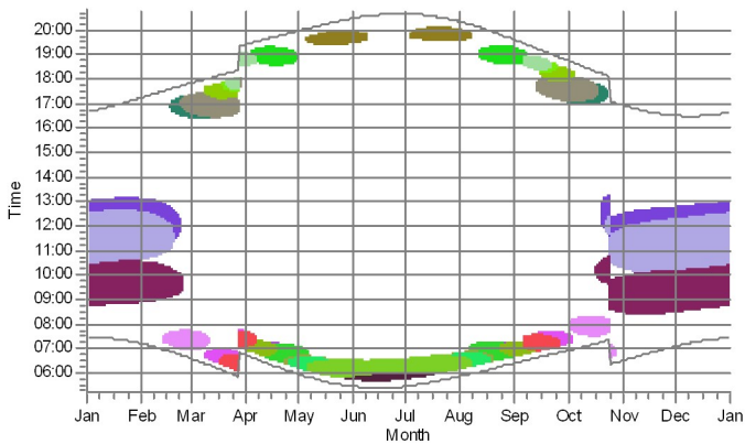
15: WTG15
