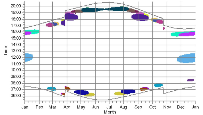
8: WTG08
