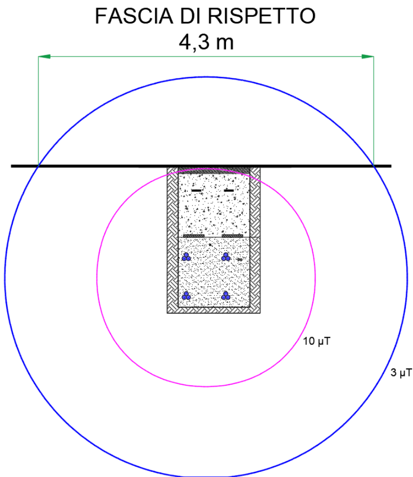
Figura 9: Curve Equicampo – Cinque Terne cavi AT – Tratta 6
