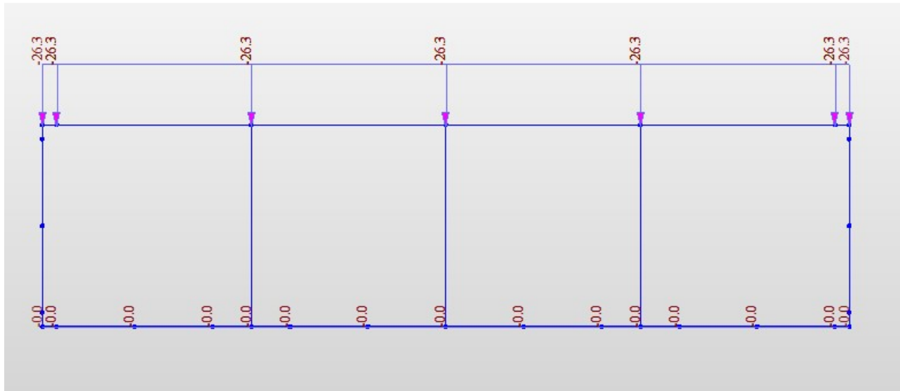
Fig. 7 – Carichi distributi verticali permanenti (PERM)
