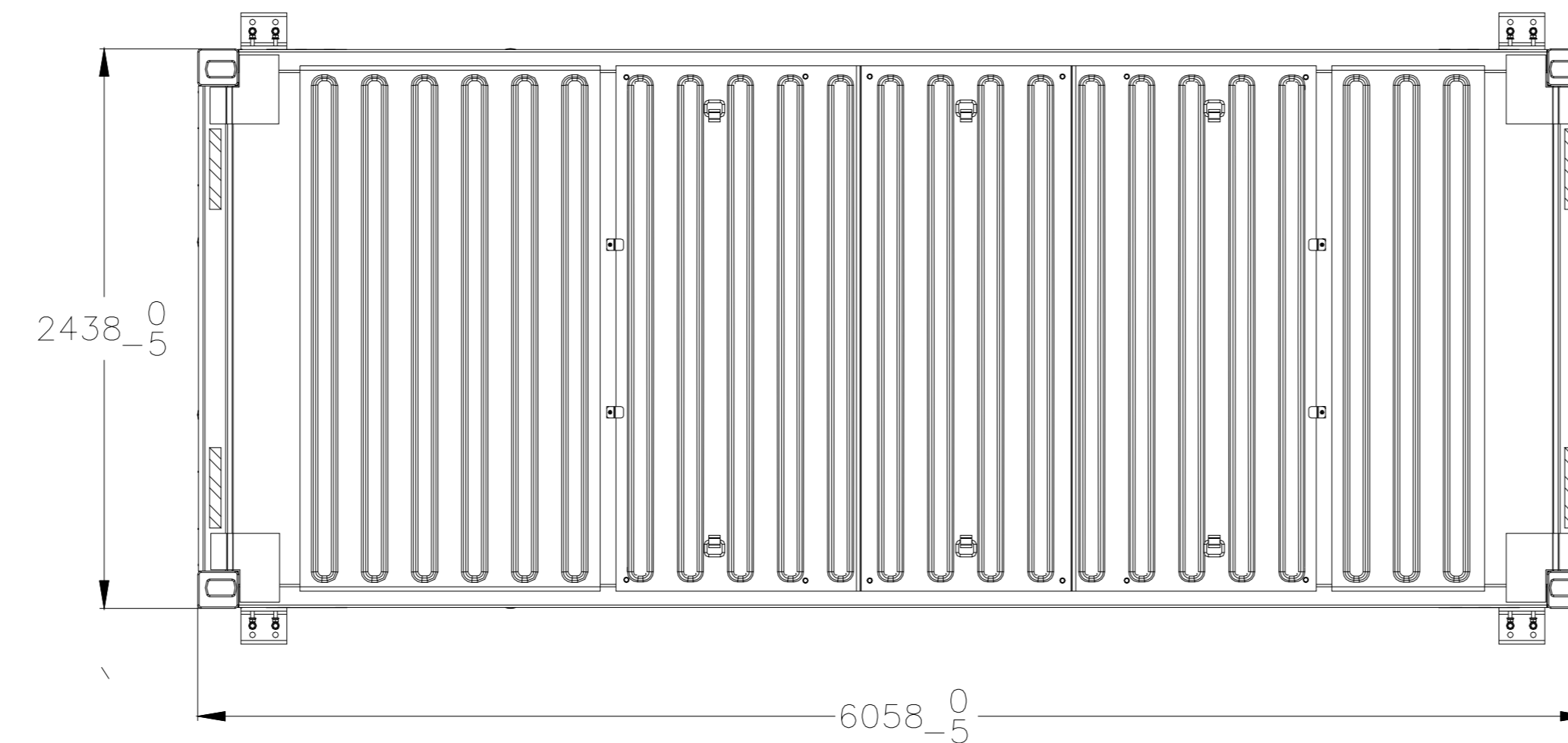
Top view
