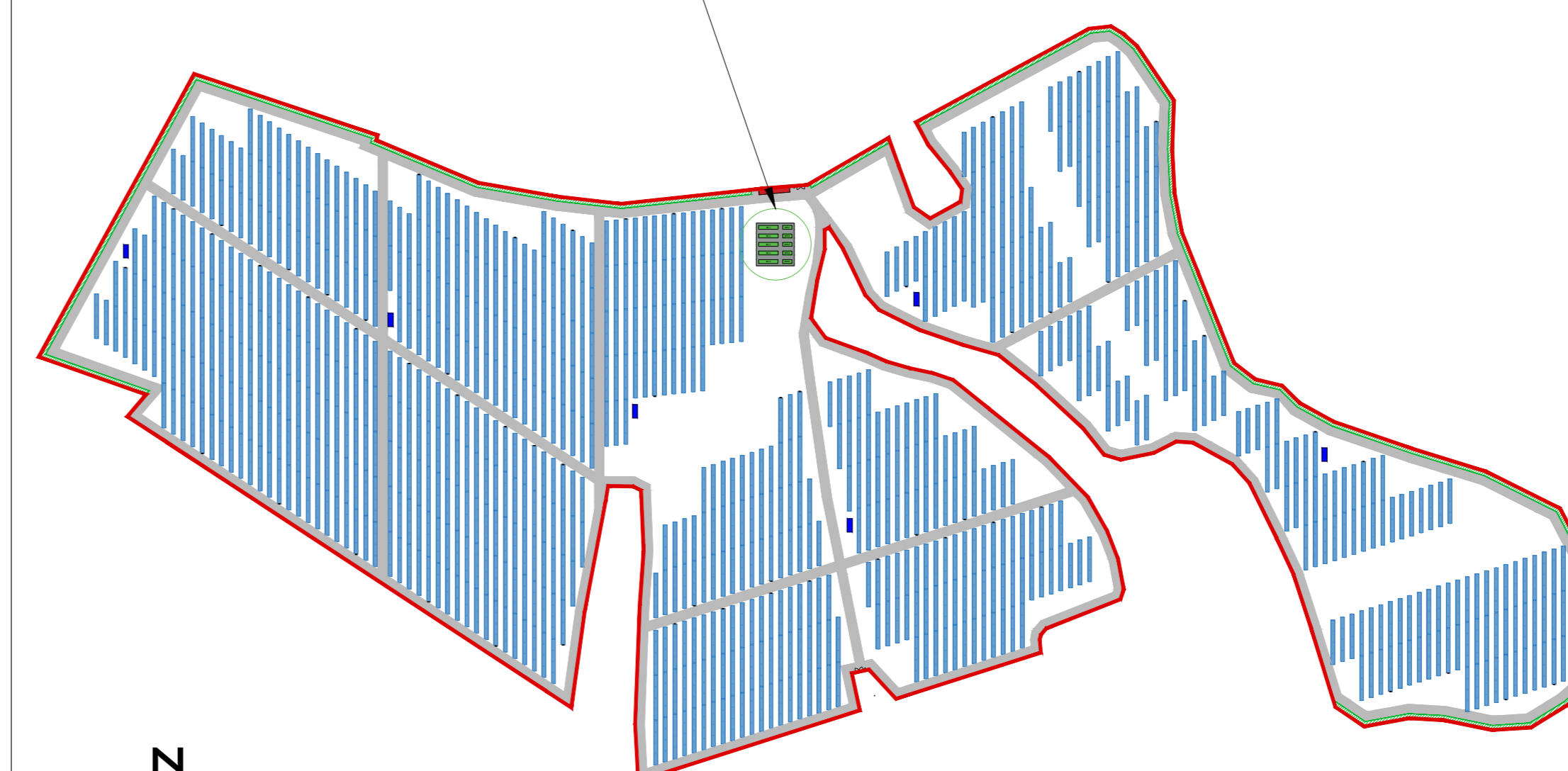
AREA IMPIANTO A - UNITA' DI ACCUMULO: 5 STORAGE CONTAINER 5 STORAGE POWER STATION
