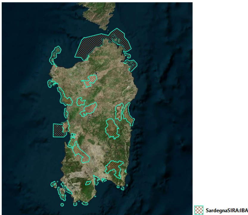
Figura 8 – Aree IBA in Sardegna
