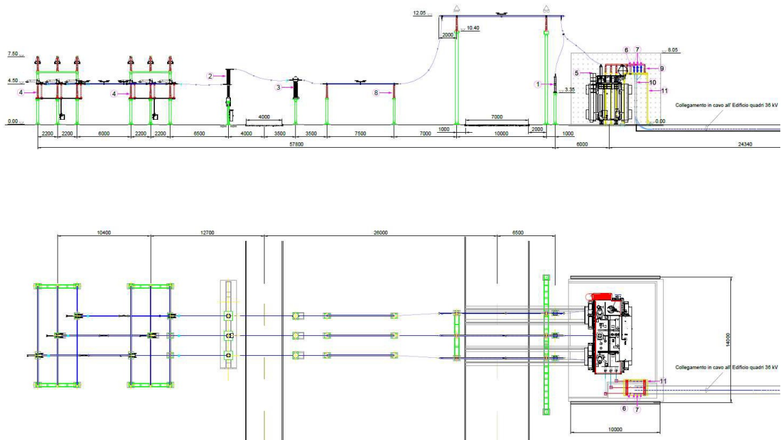
Figura 15: Stallo TR 150/36 V
