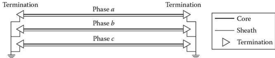
Figura 8: Schema Solid Bonding
