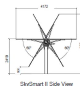
Fig. 8 – Datasheet tracker SkySmart II (ARCTECH)
