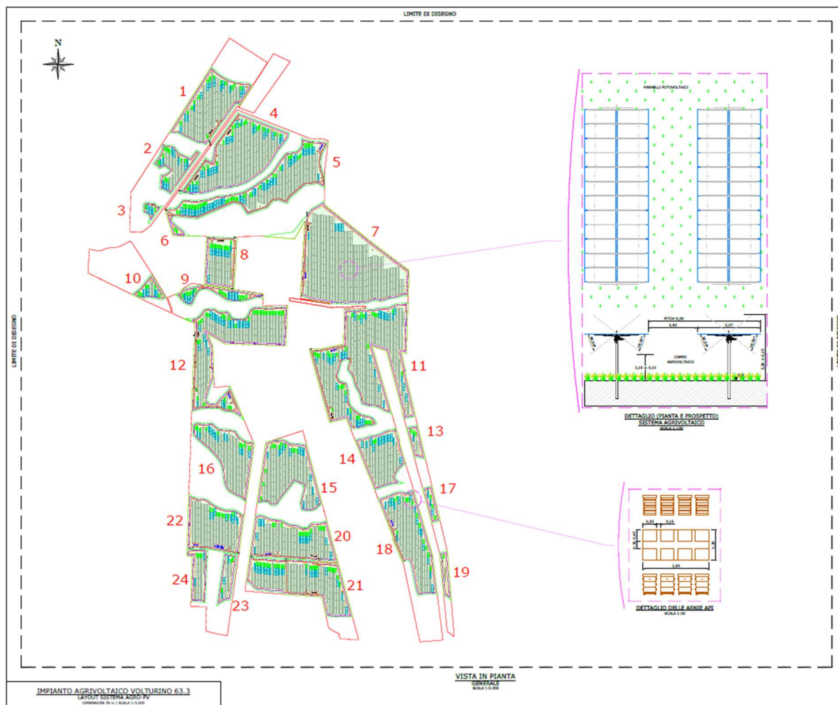
Fig. 4 – Layout Agro-PV
