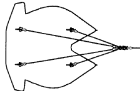
PLAN VIEW OF STEVMANTA ANCHOR
