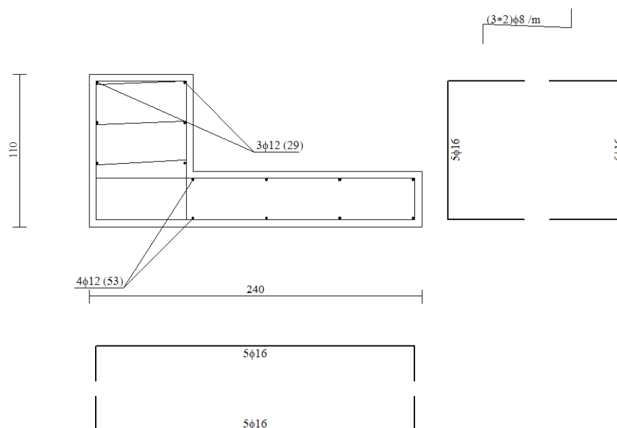
Schema armature
