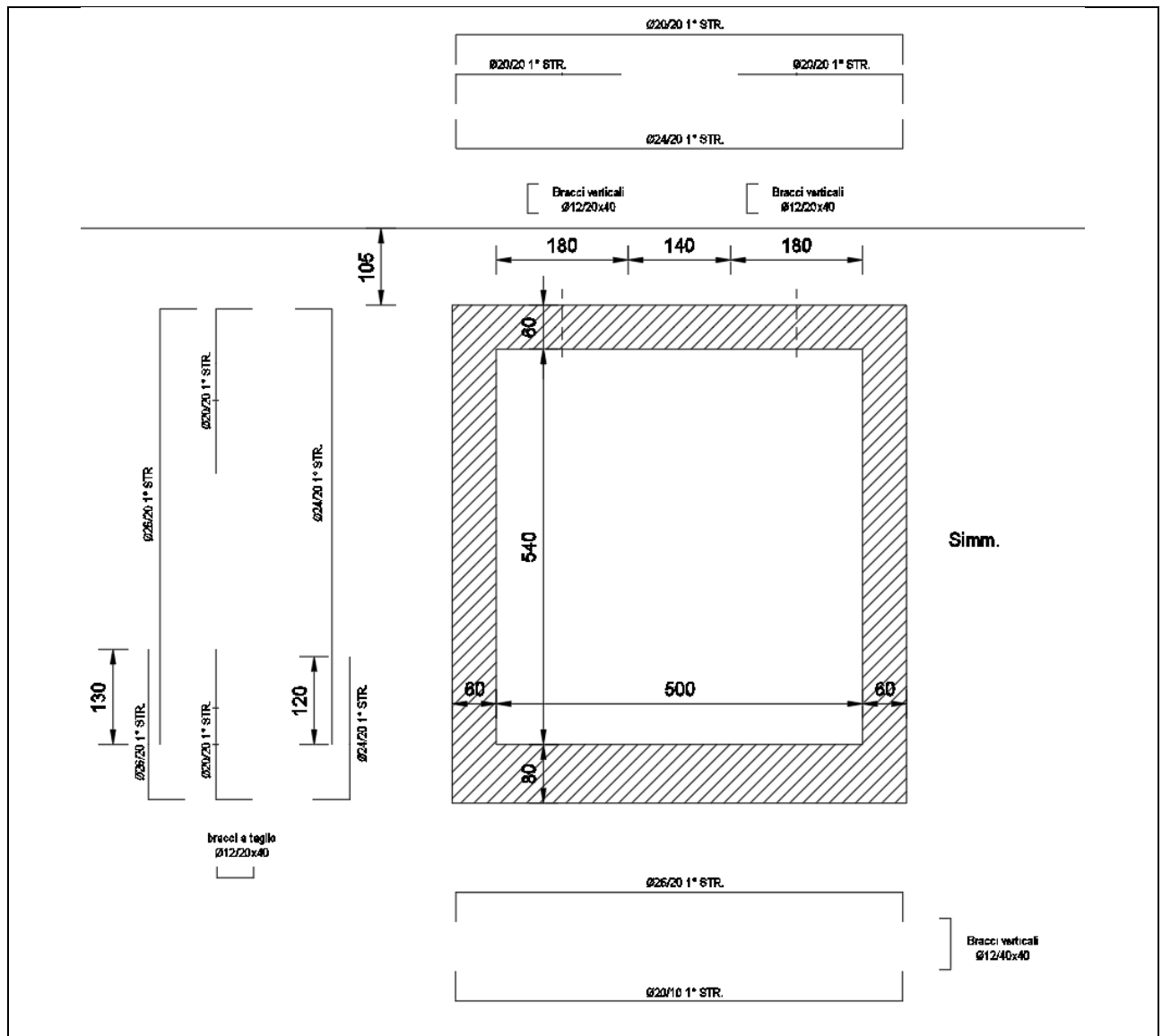
Figura 22: Schema armature
