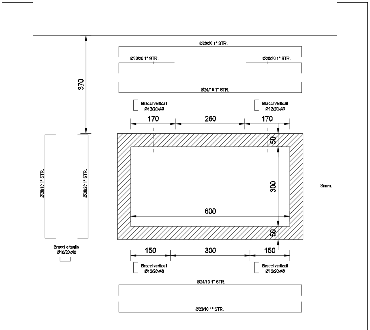
Figura 22: Schema armature
