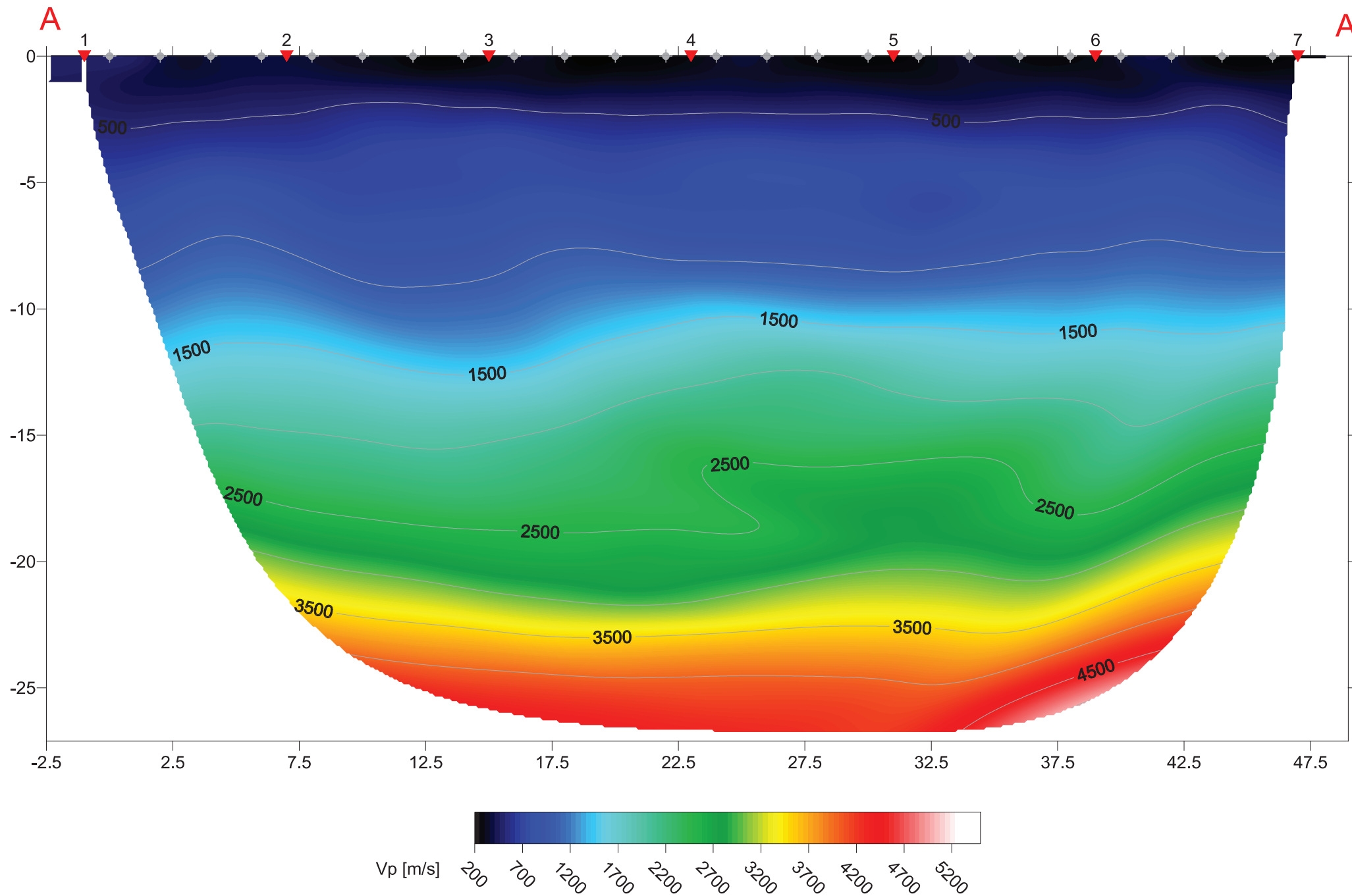
Fig. 13: Impianti Ovest (Parisi), 100 WET iterations, RMS error 1.8 %, Vp tomography model
