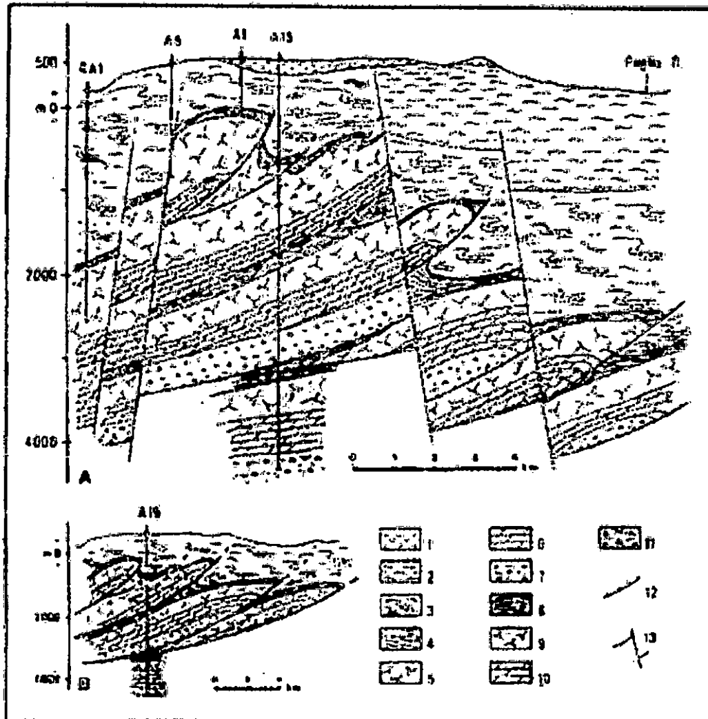
FIG. 1 - GEOLOGICAL CROSS-SECTIONS. In the section A the actual structural setting is shown; in B the Upper Fortonian one is hypothesized (see in fig. 1). 1) Volcanites (Quat.); 2) Post-orogenic Sediments (Plioc.); 3) Aquifers (Creta-Eoc.); "TUSCAN" UNITS: 4) "Scisti Policromi" (U. Creta-Eoc.); 5) Calcareous and Calcareous-Siliceous Formations (L. Lias-L. Creta); 6) "Calcarei a Rhaethavicula C." (U. Trias); 7) "Anidriti di Burano" (U. Trias); "UMBRIAN" SEQUENCES: 8) "Scaglia Canessa" and "Scaglia Rossa" (U. Creta-Gligoc.); 9) Calcareous and Calcareous-Siliceous Formations (L. Lias-L. Creta); 10) "Calcarei a Rhaethavicula C." (U. Trias); 11) "Anidriti di Burano" (U. Trias); 12) Overthrusts; 13) Tensional Faults.
