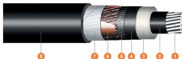
Figura 35: Cavo in alluminio AT
