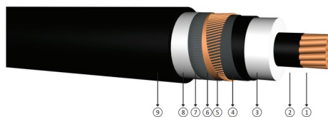
Figura 7: Cavo in rame AT
