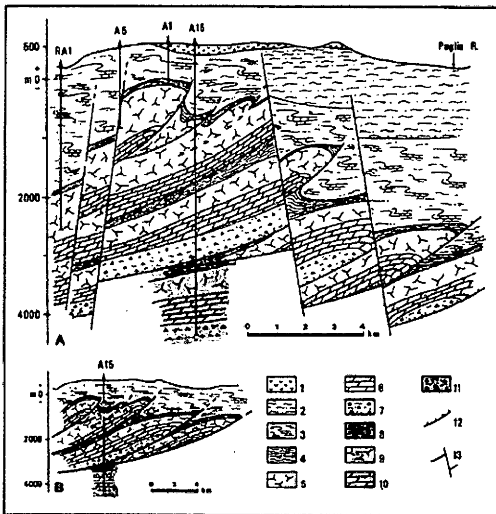
FIG.3 - GEOLOGICAL CROSS-SECTIONS. In the section A the actual structural setting is shown; in B the Upper Tortonian one is hypothesized (trace in fig.1). 1)Volcanites (Quat.); 2)Post-Orogenic Sediments (Plioc.); 3)Ligurids (Creta-Eoc.); "TUSCAN" UNITS: 4)"Scisti Policromi" (U.Creta-Eoc.); 5)Calcareous and Calcareous-Siliceous Formations (L.Lias-L.Creta); 6)"Calcari a Rhaethavicula C." (U.Trias); 7)"Anidriti di Burano" (U.Trias); "UMBRIAN" SEQUENCE: 8)"Scaglia Cinerea" and "Scaglia Rossa" (U.Creta-Oligoc.); 9)Calcareous and Calcareous-Siliceous Formations (L.Lias-L.Creta); 10)"Calcari a Rhaethavicula C." (U.Trias); 11)"Anidriti di Burano" (U.Trias); 12)Overthrusts; 13)Tensional Faults.
