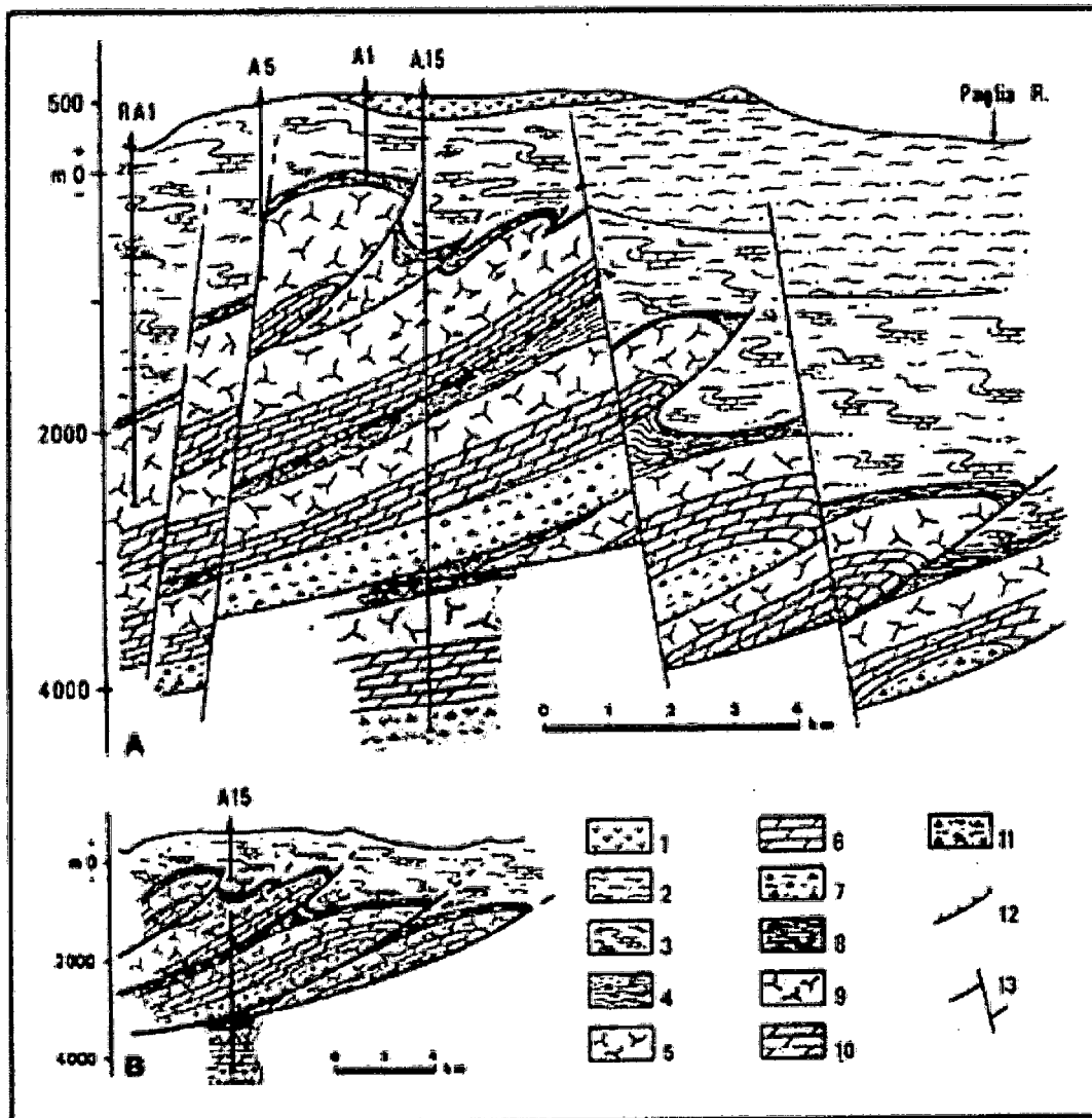
FIG.3 - GEOLOGICAL CROSS-SECTIONS. In the section A the actual structural setting is shown; in B the Upper Tortonian one is hypothesized (trace in fig.1). 1) Volcanites (Quat.); 2) Post-Orogenic Sediments (Plioc.); 3) Ligurids (Creta-Eoc.); "TUSCAN" UNITS: 4) "Scisti Policromi" (U.Creta-Eoc.); 5) Calcareous and Calcareous-Siliceous Formations (L.Lias-L.Creta); 6) "Calcari a Rhaethavicula C." (U.Trias); 7) "Anidriti di Burano" (U.Trias); "UMBRIAN" SEQUENCE: 8) "Scaglia Cinerea" and "Scaglia Rossa" (U.Creta-Oligoc.); 9) Calcareous and Calcareous-Siliceous Formations (L.Lias-L.Creta); 10) "Calcari a Rhaethavicula C." (U.Trias); 11) "Anidriti di Burano" (U.Trias); 12) Overthrusts; 13) Tensional faults.
