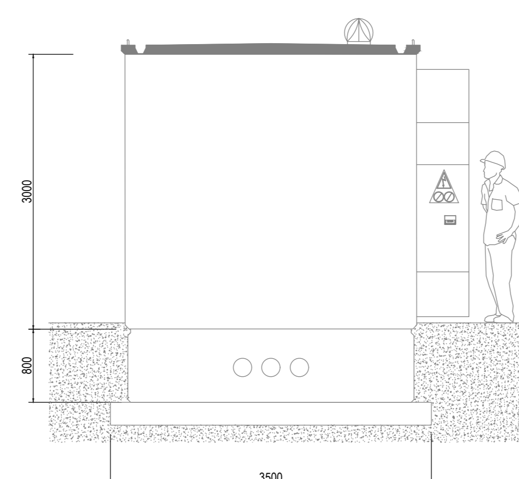
PROSPETTO C POWER STATION BESS
