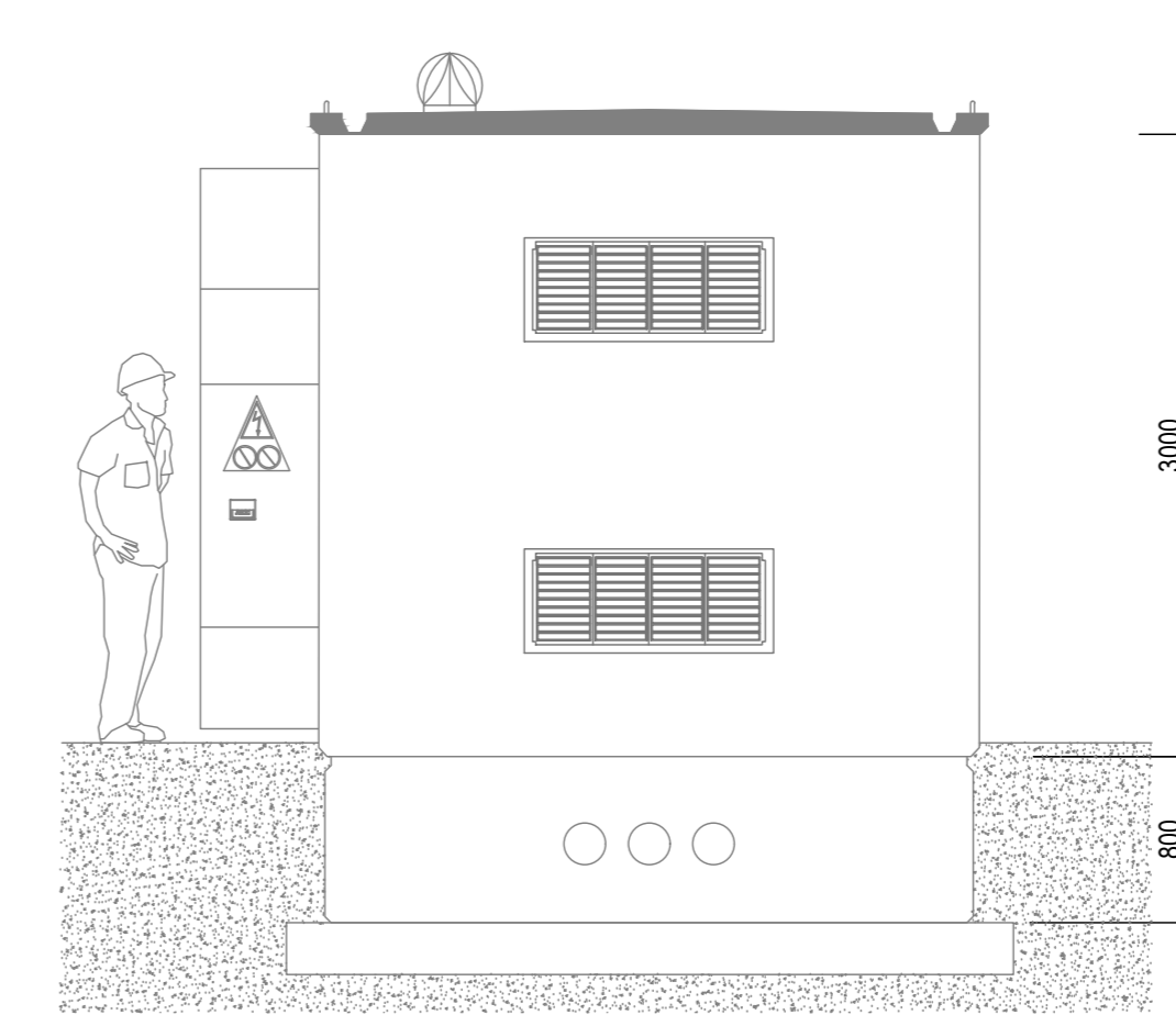
PROSPETTO D POWER STATION BESS
