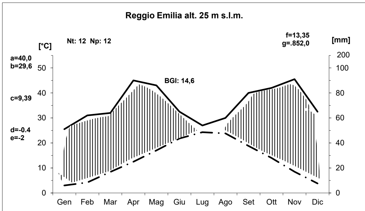
Figura 4 - Climogramma Aalter-Lieth
