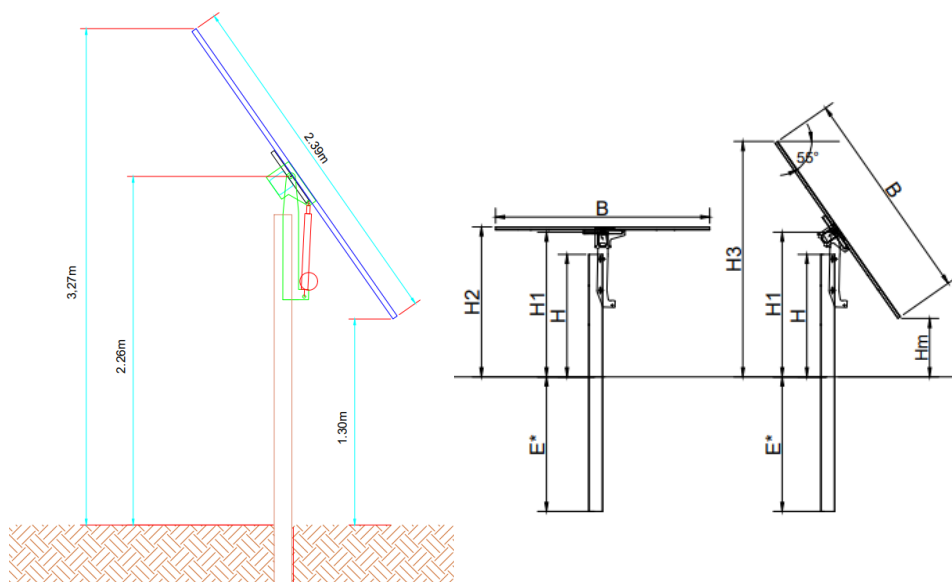
Fig.3 –Backtracking
