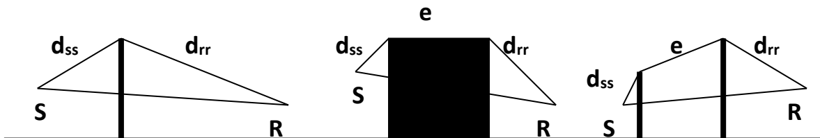
Fig. 9- Barriere, ISO 9613-2
