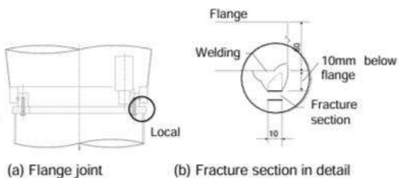
Fig. 2 Detail drawing of fracture section
