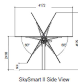
Fig. 2 – Datasheet tracker SkySmart II (ARCTECH)
