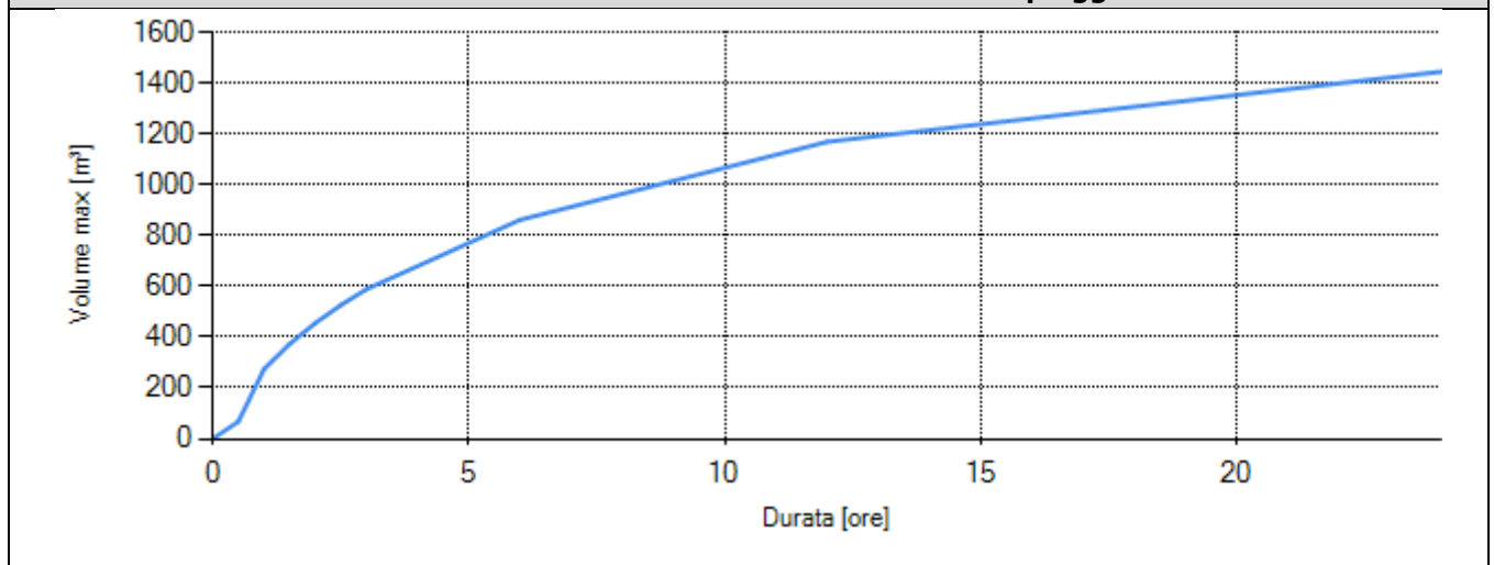
Variation volume maximum invaded in function of the duration of the rain - Graph
